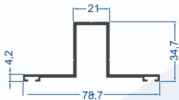
Insulating Glass Middle Mullion Profile
