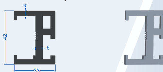
Top Rail Profile
