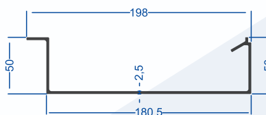
Stream Bottom Profile
