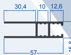
Single Glass Flat
