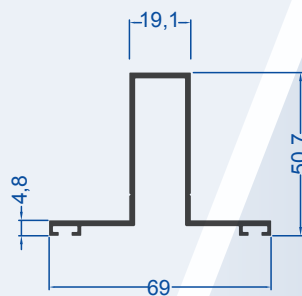
Single Glazing Center Profile
