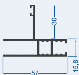
Single Wing Gasket & Clamped Sash Profile
