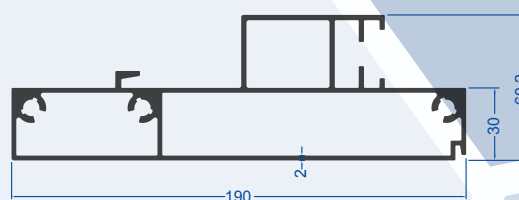
Additional Profile of the Stream
