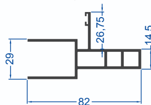
Insulating Glass Gasket & Clamped Sash
