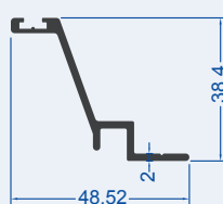
Front Support Profile
