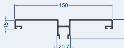
Top Case Profile
