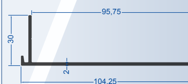
Stream Raising Profile
