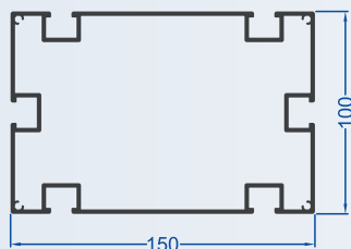
Base Profile 100x150cm
