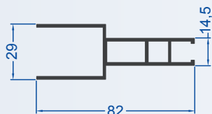
Insulating Glass Flat Sash
